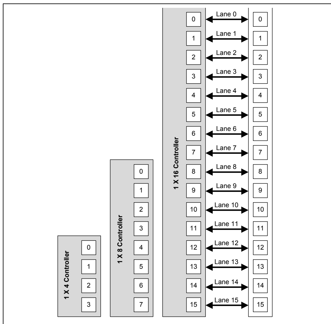
Figure 2-5. PCI Express* Typical Operation 16 Lanes Mapping
