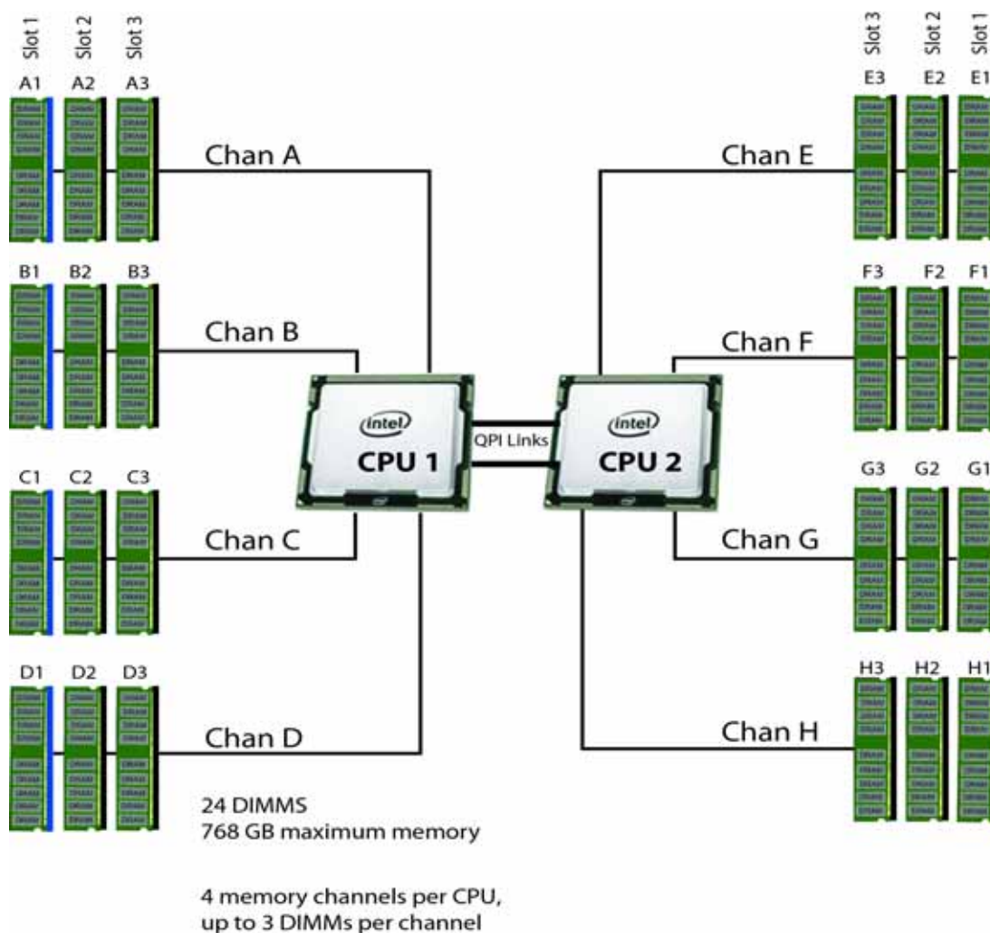
Figure 3 UCS B200 M4 Memory Organization
